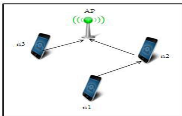
Fig 3. Redundant Elimination
